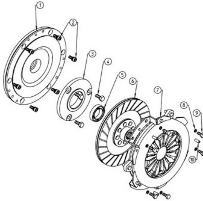
11 KIT EMBRAGUE / CLUTCH KIT
